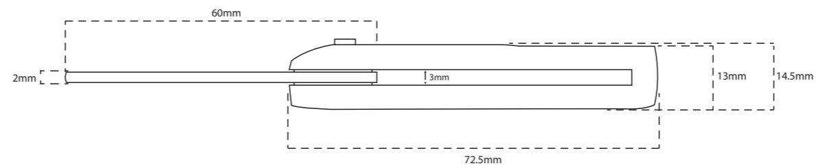
Side view of the Flix DS
